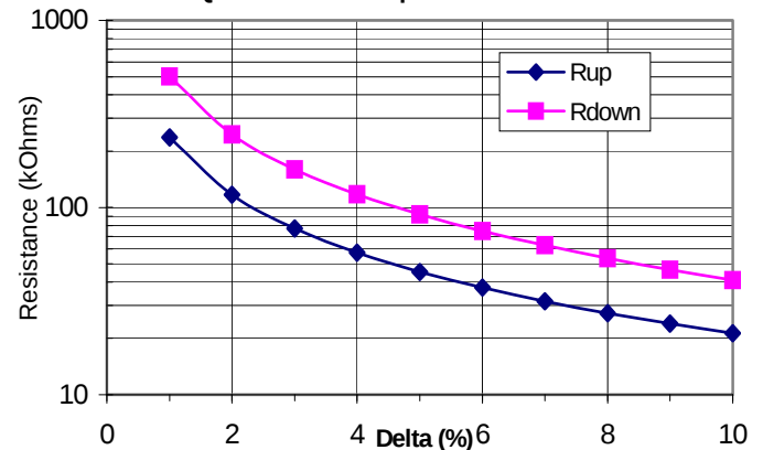
QHS50-015 Trim-up and Trim-down Resistance
