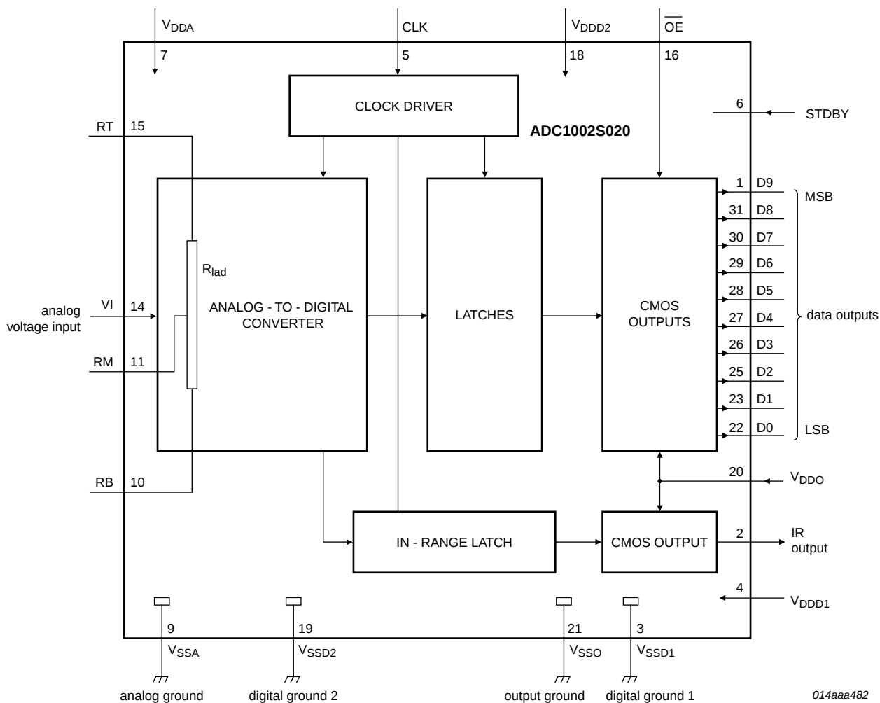
Fig 1. Block diagram
