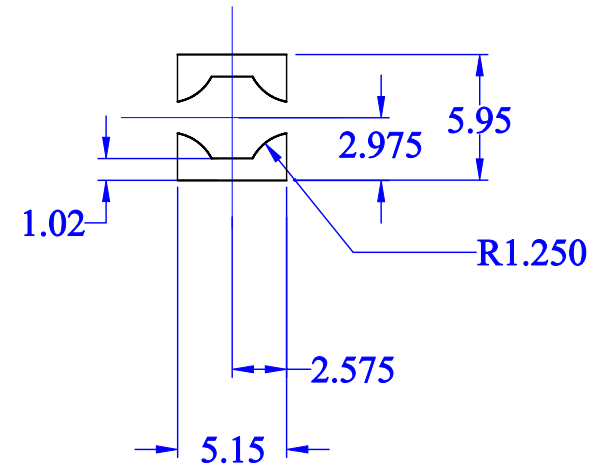
2 PAD LAYOUT
