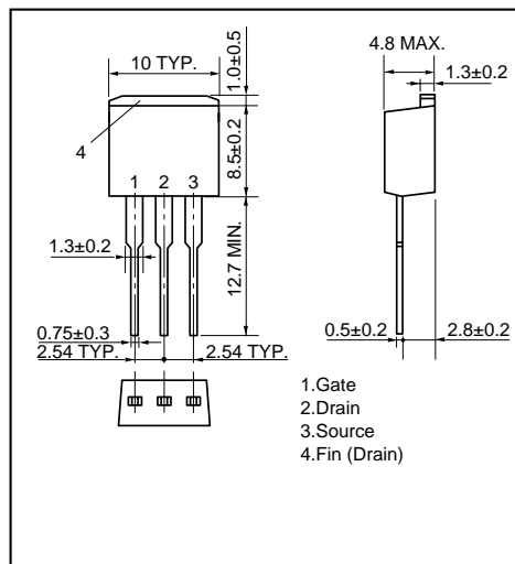
4) TO-220SMD(MP-25Z) Note
