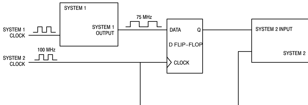
Figure 12. System Example
