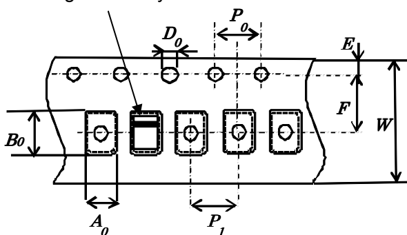
Fig.4 Emboss Carrier Tape Dimensions
