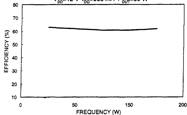
DRAIN EFFICIENCY vs FREQUENCY
