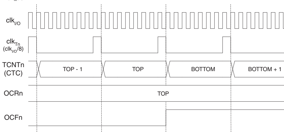
Figure 44. Timer/Counter Timing Diagram, Clear Timer on Compare Match Mode, with Prescaler ( f_{clk\_I/O}/8 )
