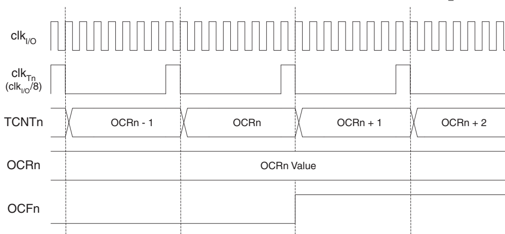
Figure 43. Timer/Counter Timing Diagram, Setting of OCF0, with Prescaler ( f_{clk\_I/O}/8 )
