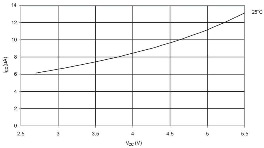
Figure 179. Power-Save Supply Current vs. V_{CC} (Watchdog Timer Disabled)
