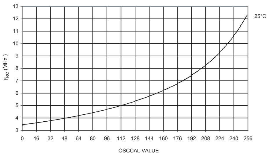
Figure 213. Calibrated 8 MHz RC Oscillator Frequency vs. OSCCAL Value
