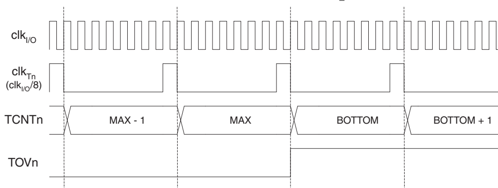
Figure 42. Timer/Counter Timing Diagram, with Prescaler ( f_{clk\_I/O}/8 )
