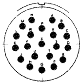
22-21 21 NO.16 CONTACTS
