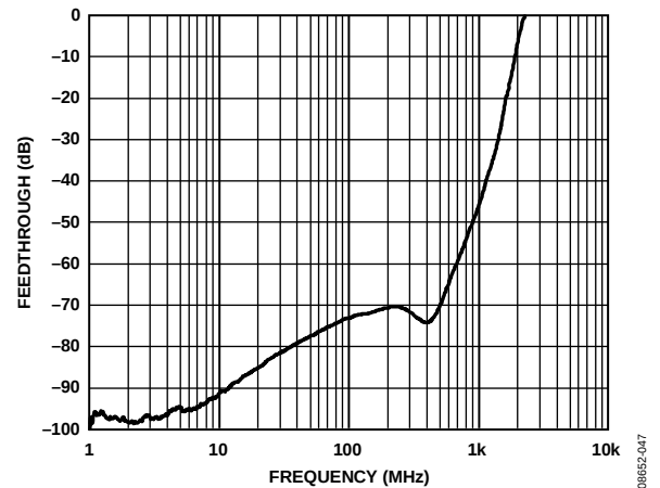
Figure 41. ADV3222 Off Isolation
