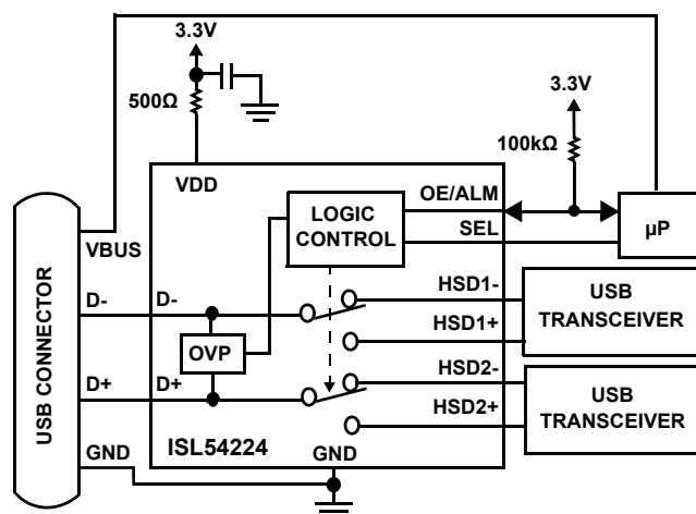
FIGURE 1. TYPICAL APPLICATION
