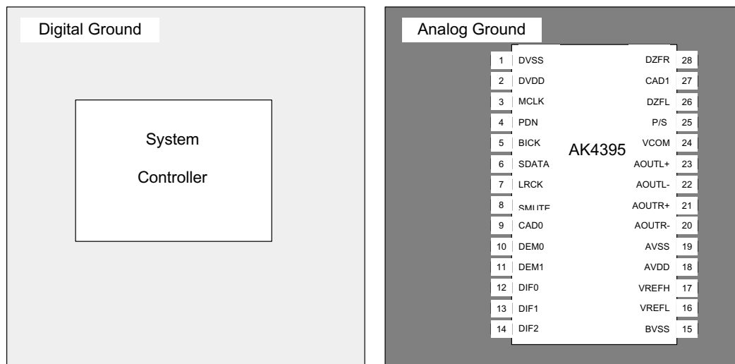
Figure 11. Ground Layout
