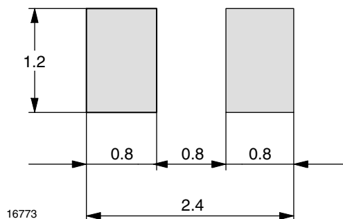
Fig. 11 - Recommended Foot Pads (in mm)
