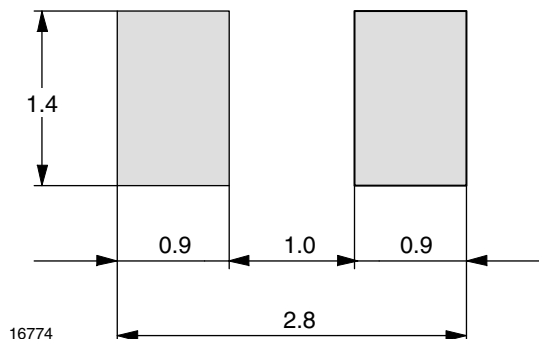
Fig. 12 - Recommended Foot Pads (in mm)
