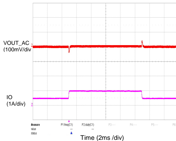
Load Transient (I OUT =0.5A to 1A)
