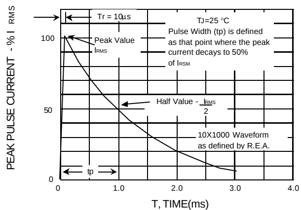
FIG.5 - PULSE WAVEFORM
