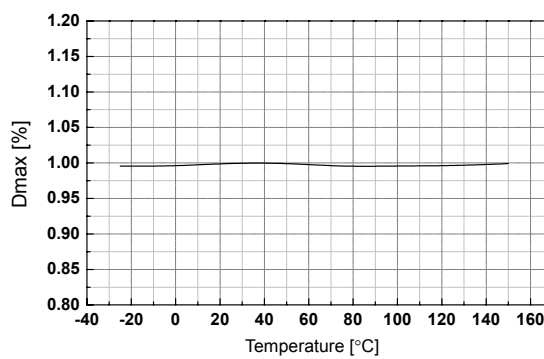
Figure 6. Maximum Duty Cycle vs. Temp.
