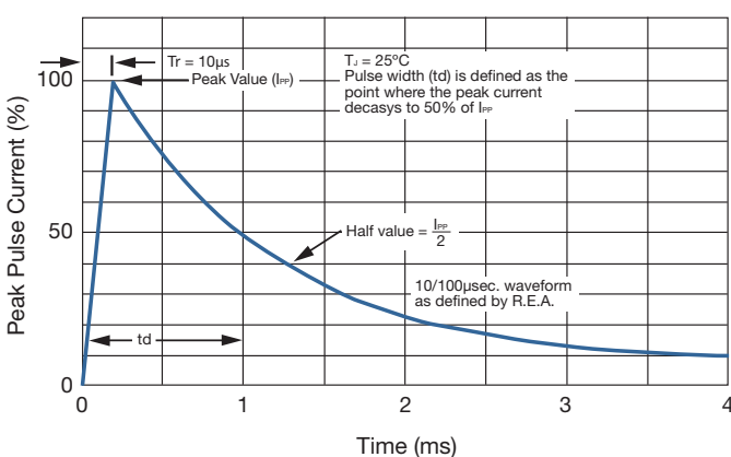
FIG 5. PULSE WAVEFORM
