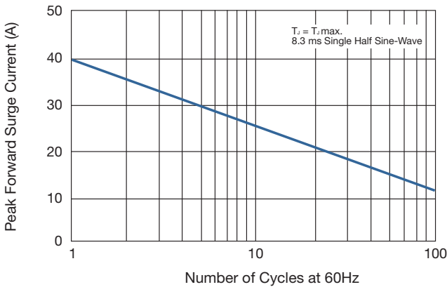
FIG 2. MAXIMUM NON-REPETITIVE
