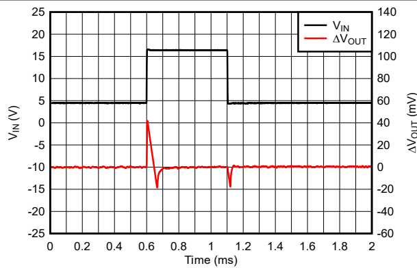
Figure 7-10. TPS77033 Line Transient Response (New Chip)
