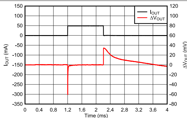
Figure 7-12. TPS77033 Load Transient Response (Legacy Chip)
