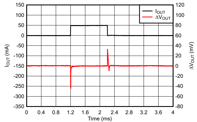
Figure 7-11. TPS77015 Load Transient Response (Legacy Chip)
