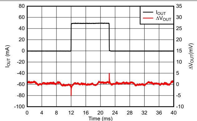
Figure 7-13. TPS77033 Load Transient Response (New Chip)
