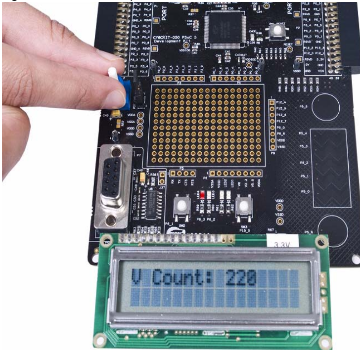
Figure 5-11. ADC Output
