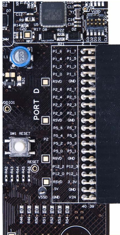
Figure 4-8. Port D
