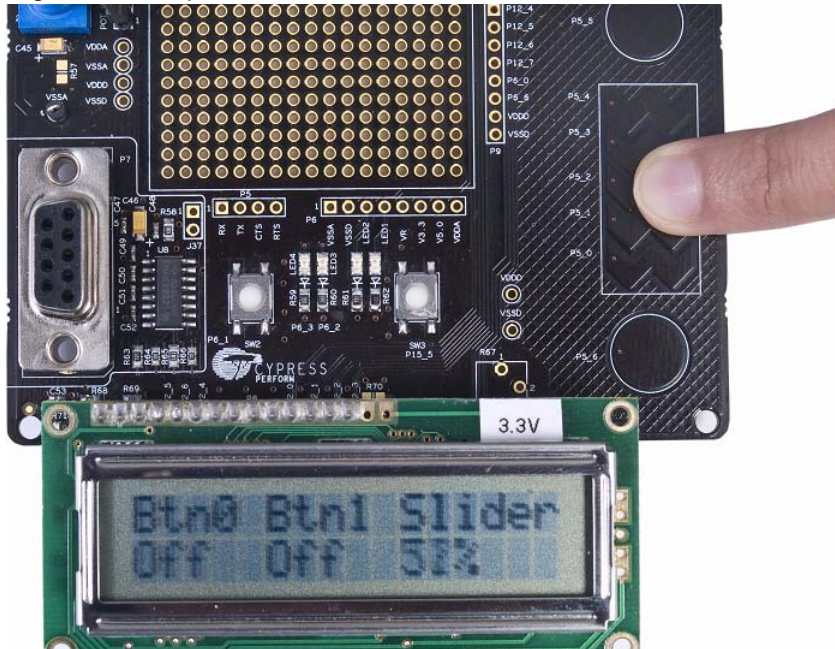
Figure 5-9. CapSense Slider
