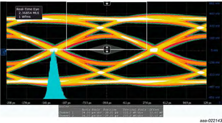
Test frequency: 148.5 MHz Differential swing voltage: 849 mV Horizontal scale: 34 ps/div Remark: Measured at Test Point 2 (TP2) worst cable emulator, reference cable equalizer and worst case positive skew.
