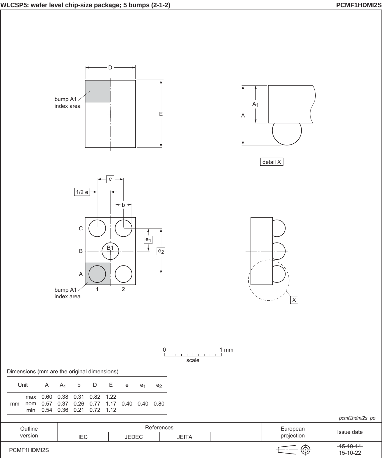
Fig 19. Package outline WLCSP5
