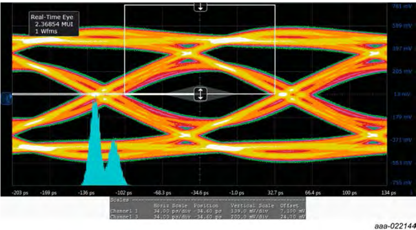
Test frequency: 148.5 MHz Differential swing voltage: 909 mV Horizontal scale: 34 ps/div Remark: Measured at Test Point 2 (TP2) worst cable emulator, reference cable equalizer and worst case positive skew.
