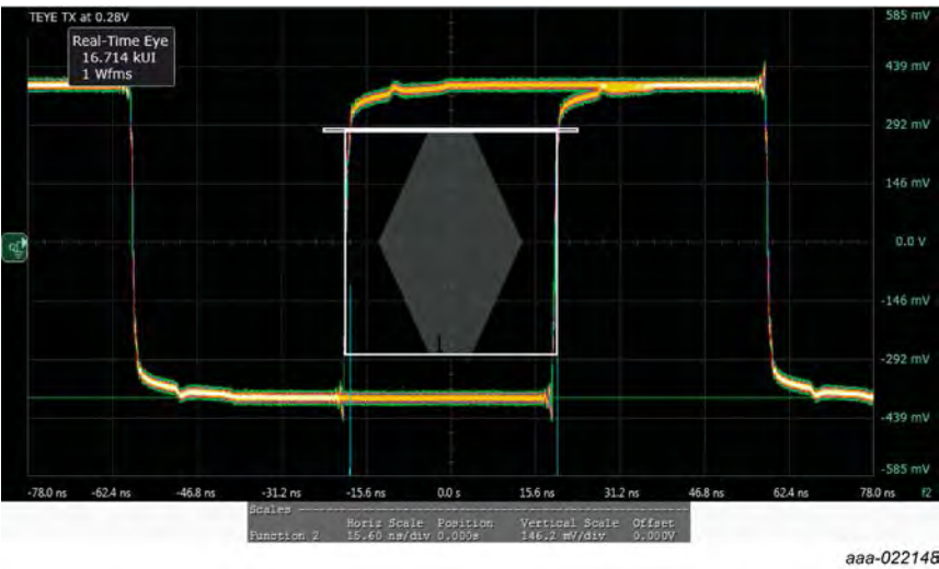
Fig 9. MIPI M-PHY PWM-TX transmitter eye opening at 140 mV, test board with PCMF2HDMI2S; typical values
