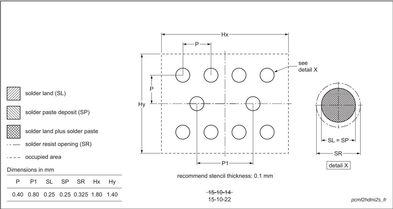
WLCSP10: Solder footprint and stencil aperture
