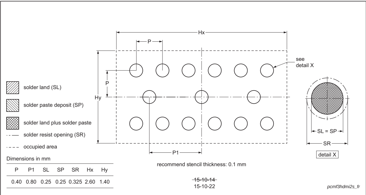
WLCSP15: Solder footprint and stencil aperture
