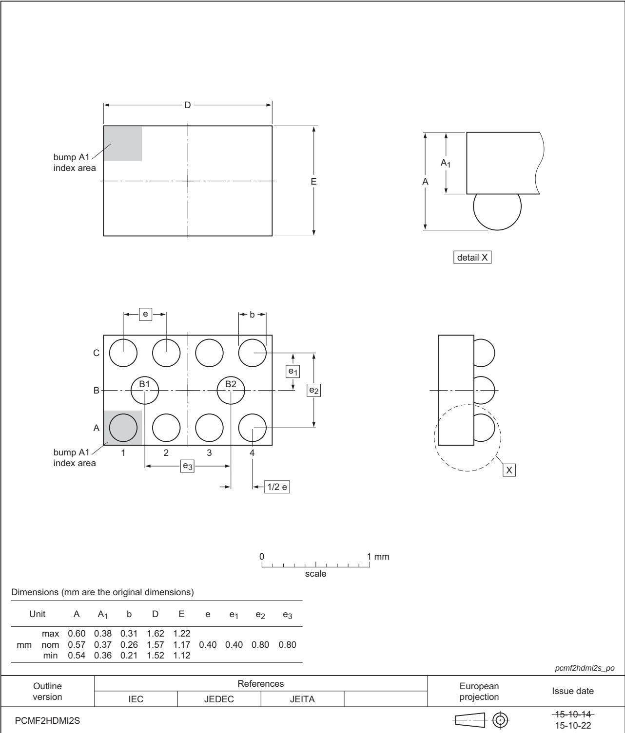
Fig 20. Package outline WLCSP10
