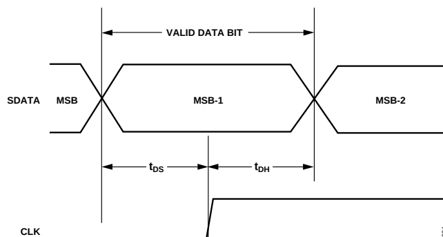
Figure 4. SDATA Timing
