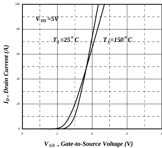
Fig 11. Transfer Characteristics
