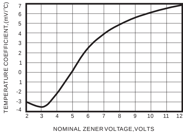
Fig.1 TEMPERATURE COEFFICENTS
