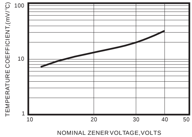
Fig.2 TEMPERATURE COEFFICENTS
