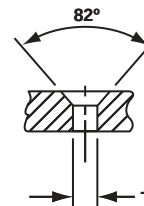
GT020RFSM Countersunk holes required when mating with GT06CFGG, page 55 and GT08CFGG, page 73
