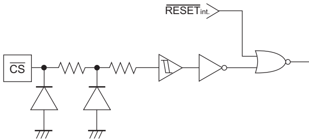
Fig.58 CS input equivalent circuit
