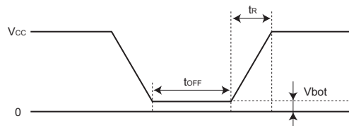
Fig.64 Rise waveform
