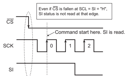
Fig.45 Operating timing
