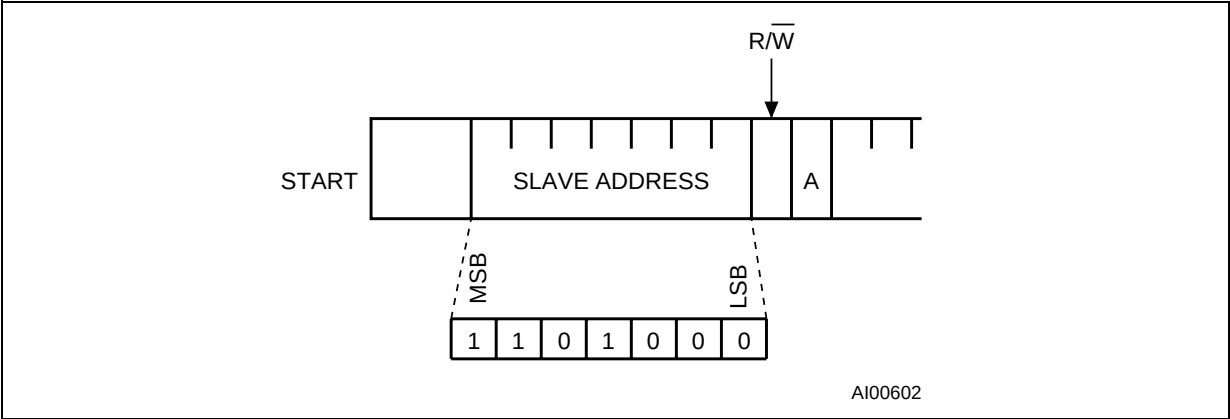
Figure 12. READ Mode Sequence
