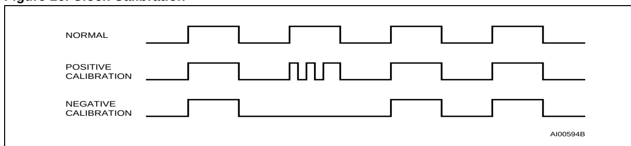
Figure 16. Clock Calibration
