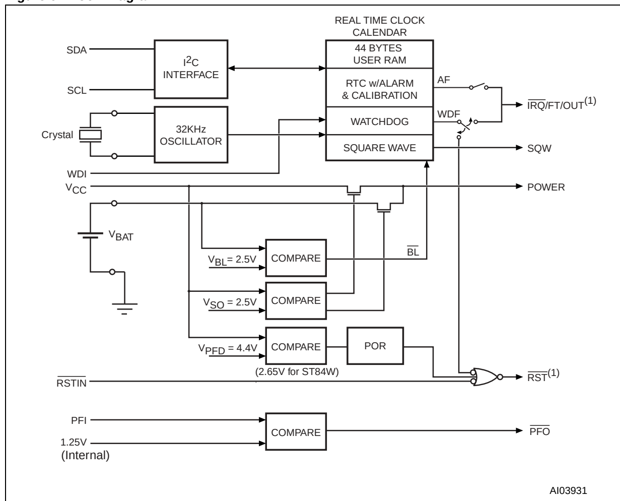
Figure 6. Block Diagram
