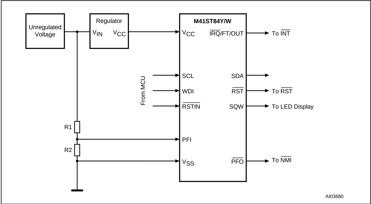
Figure 7. Hardware Hookup
