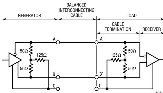
Figure 19. Typical V.35 Interface
