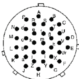
Shell Size 22 35
