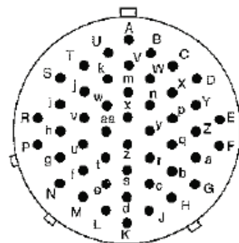
Shell Size 24 48
