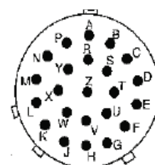
Shell Size 18 23
