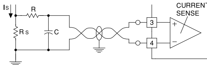
Figure 5. Current-Sense Amplifier Connections
