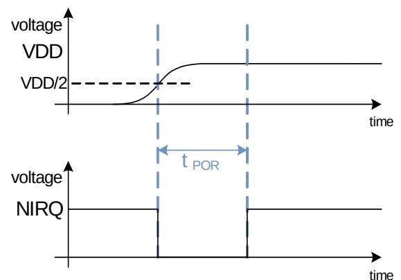
Figure 14. Power-up, NIRQ
