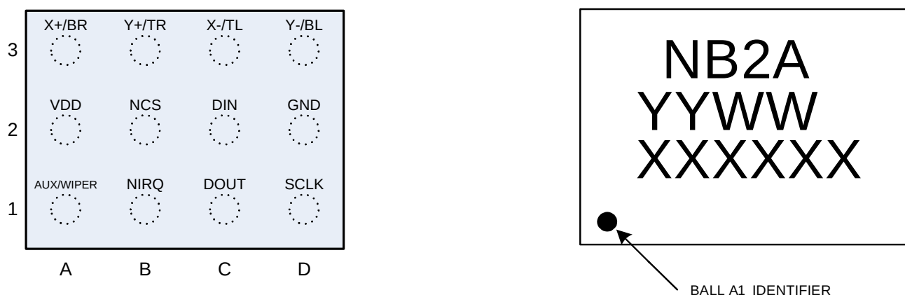
Figure 2. SX8653 WLCSP Top View, Solder Bumps on Bottom Side
