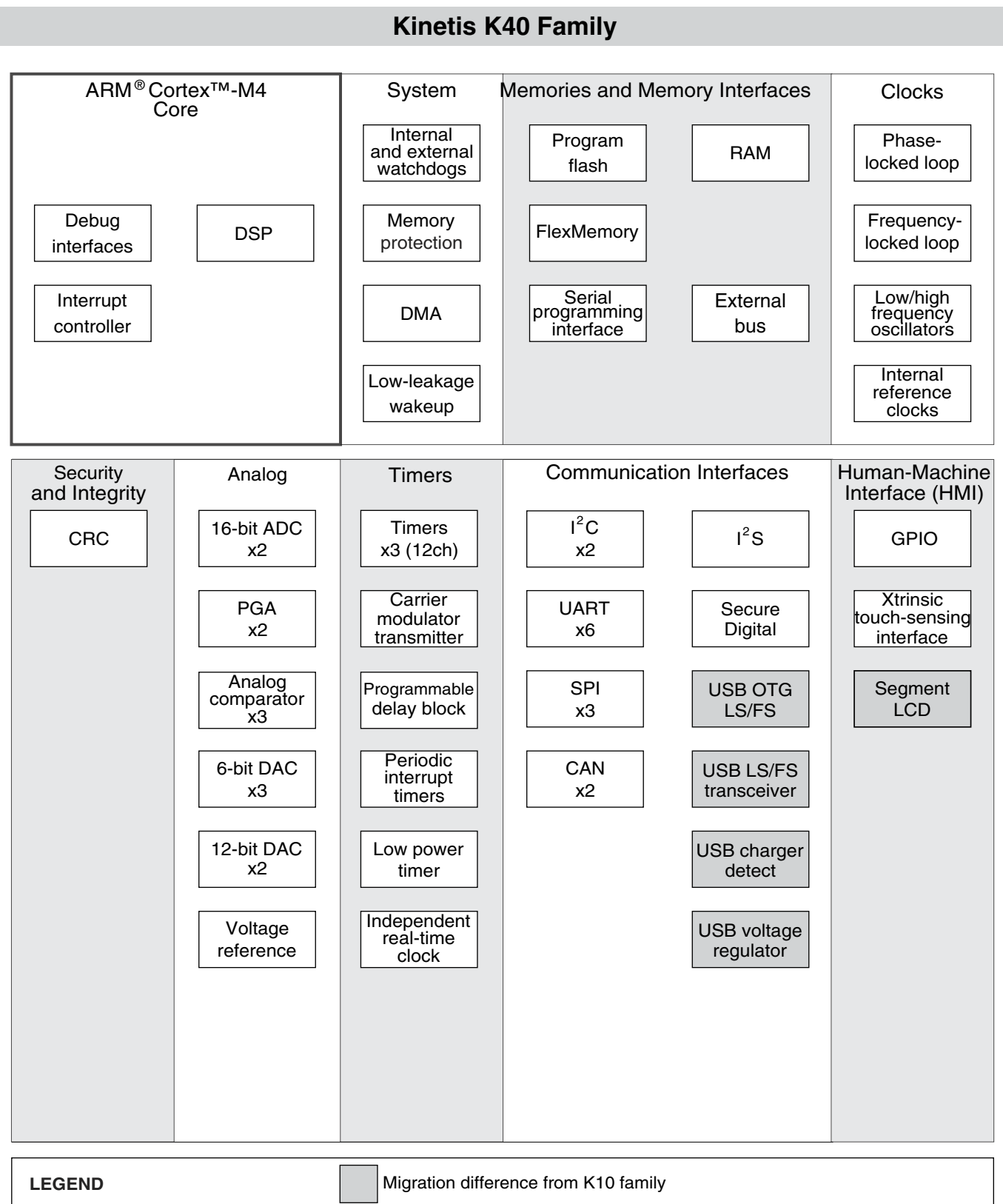
Figure 2. K40 Block Diagram
