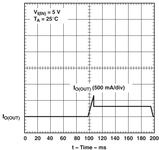
Figure 7. TPS2010A, Ramped Load on Enabled Device
