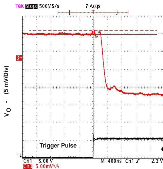
WORST-CASE GLITCH
