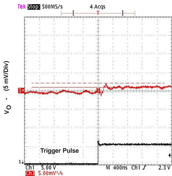
MIDSCALE GLITCH
