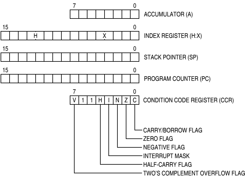
Figure 7-1. CPU Registers
