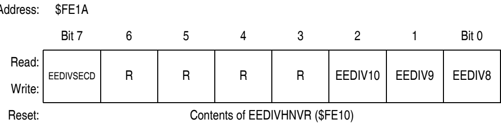
Figure 5-5. EEPROM Divider Register High (EEDIVH)
