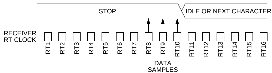
Figure 15-8. Fast Data
