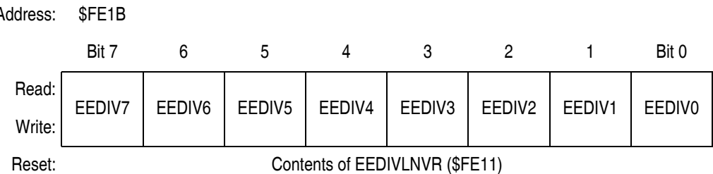
Figure 5-6. EEPROM Divider Register Low (EEDIVL)
