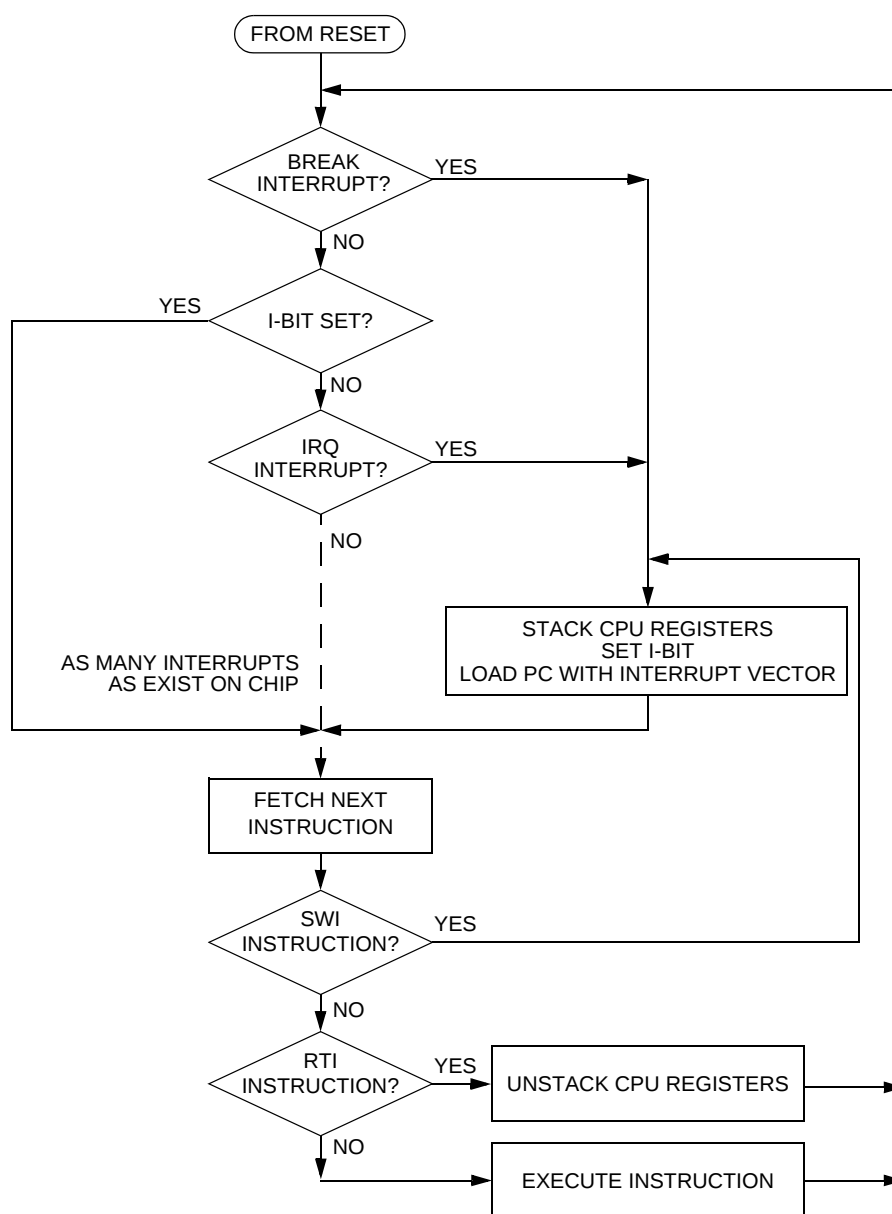
Figure 8-10. Interrupt Processing
