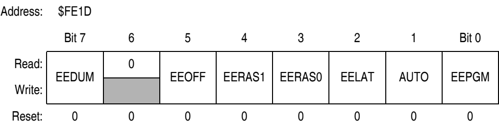
Figure 5-2. EEPROM Control Register (EECR)
