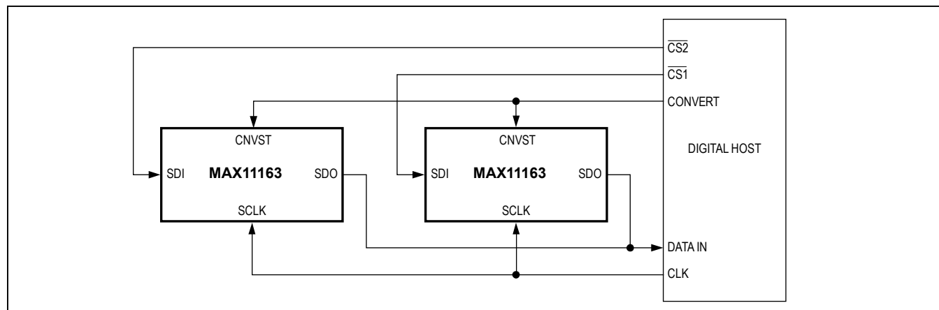
Figure 9. \overline{\text{CS}} Mode 4-Wire, No-Busy Indicator Connection Diagram
