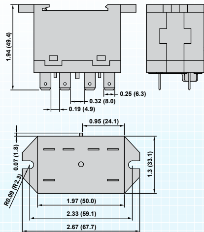
C3 – PANEL/DIN MOUNT (QC/SOLDER TERMINAL)
