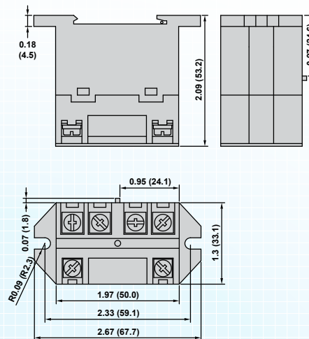
C3 – PANEL/DIN MOUNT (SCREW TERMINAL)
