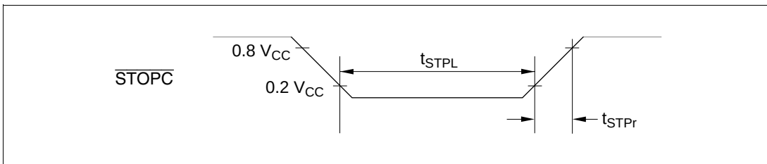
Figure 25-16 \overline{\text{STOPC}} Timing (HD404318 Series)
