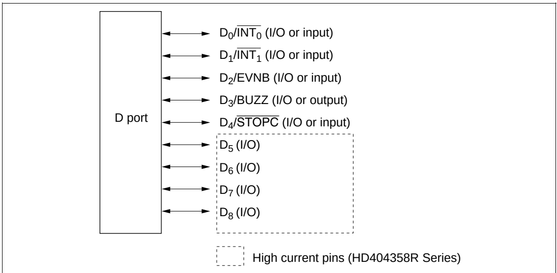
Figure 10-1 D Port Structure
