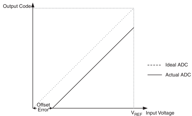
Figure 23-10. Offset Error
