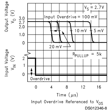
Response Time for Various Input Overdrives -t_{PHL}
