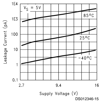
Leakage Current vs Supply Voltage
