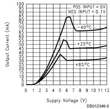
Output Sinking Current vs Supply Voltage
