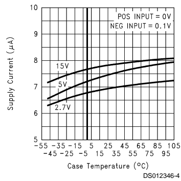
Supply Current vs Temperature while Sinking
