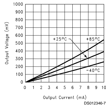
Output Sinking Current vs Output Voltage @ 15V
