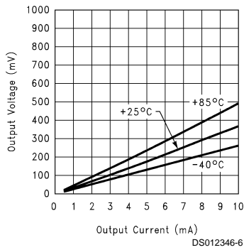
Output Sinking Current vs Output Voltage @ 5V
