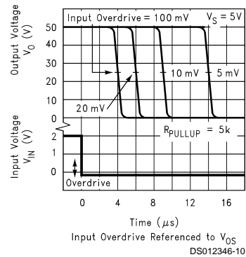
Response Time vs Various Input Overdrives -t_{PHL}
