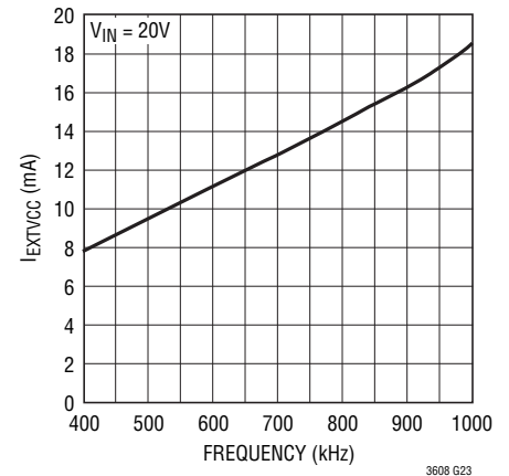
I_{\text{EXTVCC}} vs Frequency
