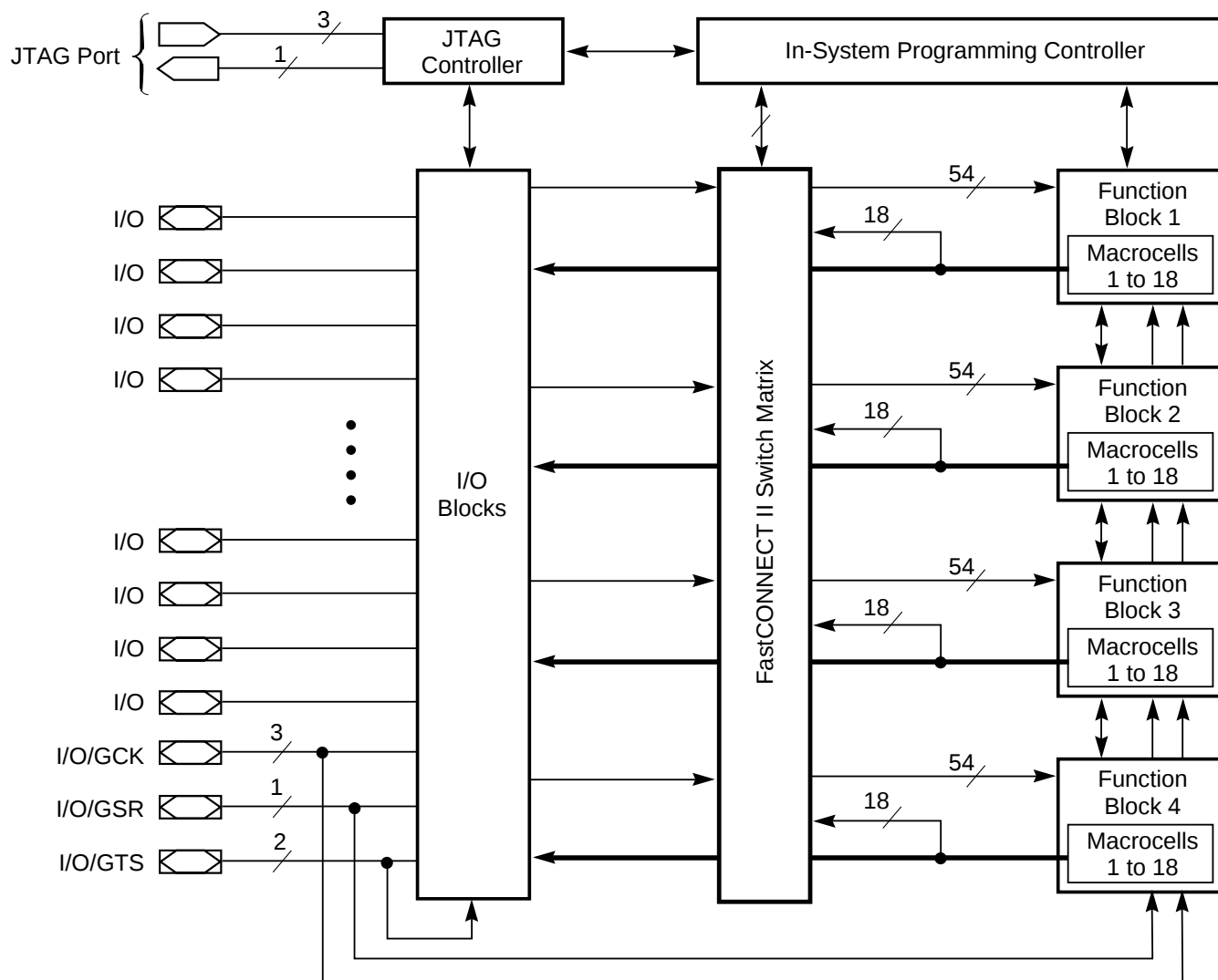
Figure 2: XC9572XV Architecture
