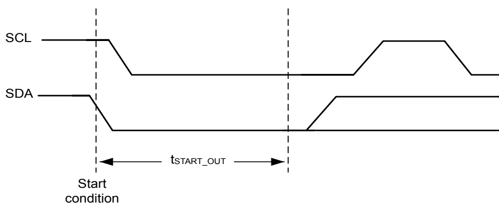
Figure 25. I 2 C timeout on Start condition
