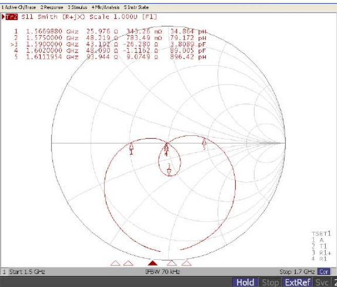
Fig. 4 Smith Chart
