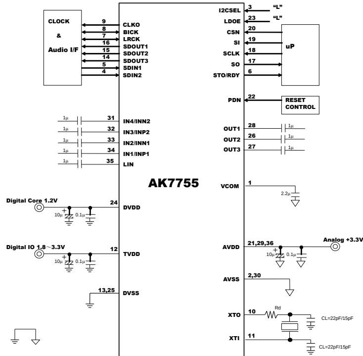
Figure 79. Serial Interface Connection with External Power Supply
