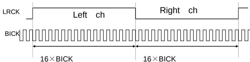
Figure 21. BITFS[1:0] bits = 2h(32fs) (LRIF[1:0]bits = 0h)
