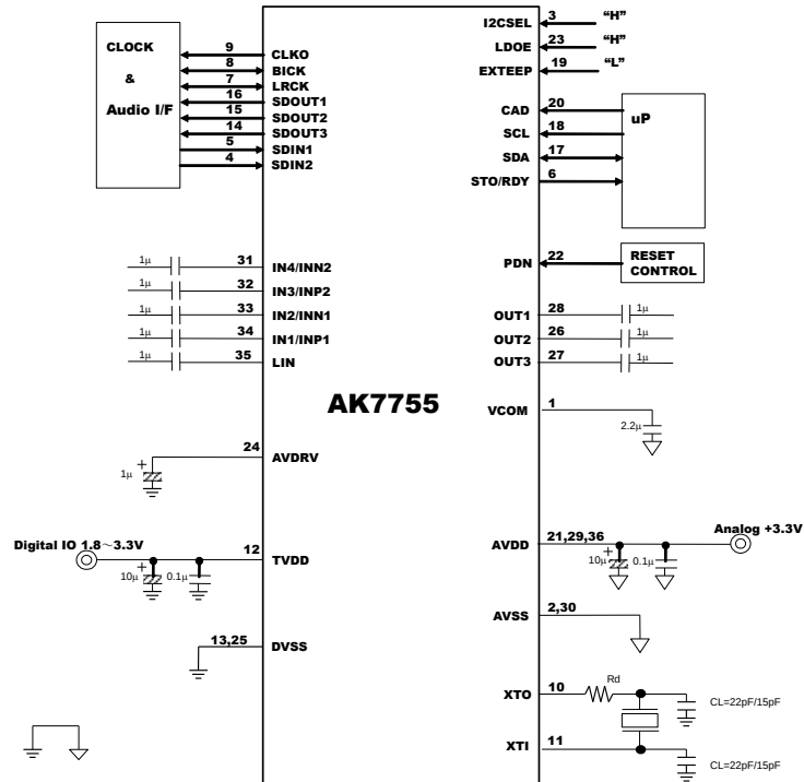
Figure 82. I 2 C Interface Connection with Internal LDO
