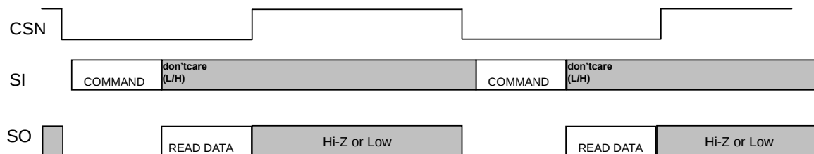
Figure 52. Read Sequence2 in Echo Back Mode (SPI)
