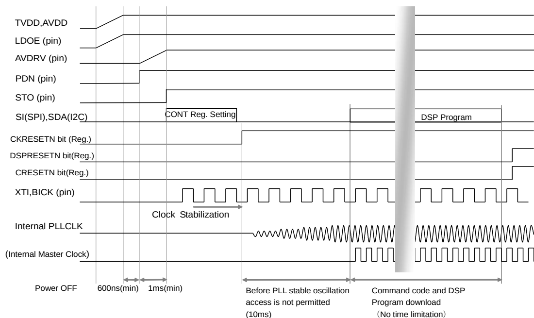
Figure 28. Power-up Sequence 5 (With LDO (LDOE pin = “H”), No downloading from EEPROM)
