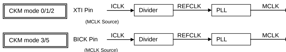
Figure 16. Relation Ship between ICLK and MCLK
