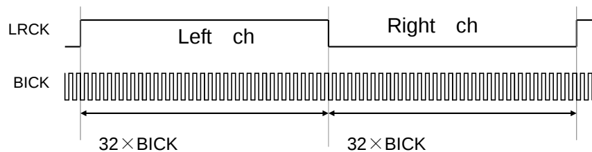
Figure 19. BITFS[1:0] bits = 0h(64fs) (LRIF[1:0]bits = 0h)
