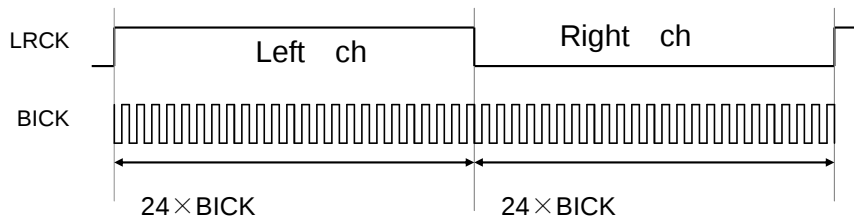
Figure 20. BITFS[1:0] bits = 1h(48fs) (LRIF[1:0]bits = 0h)
