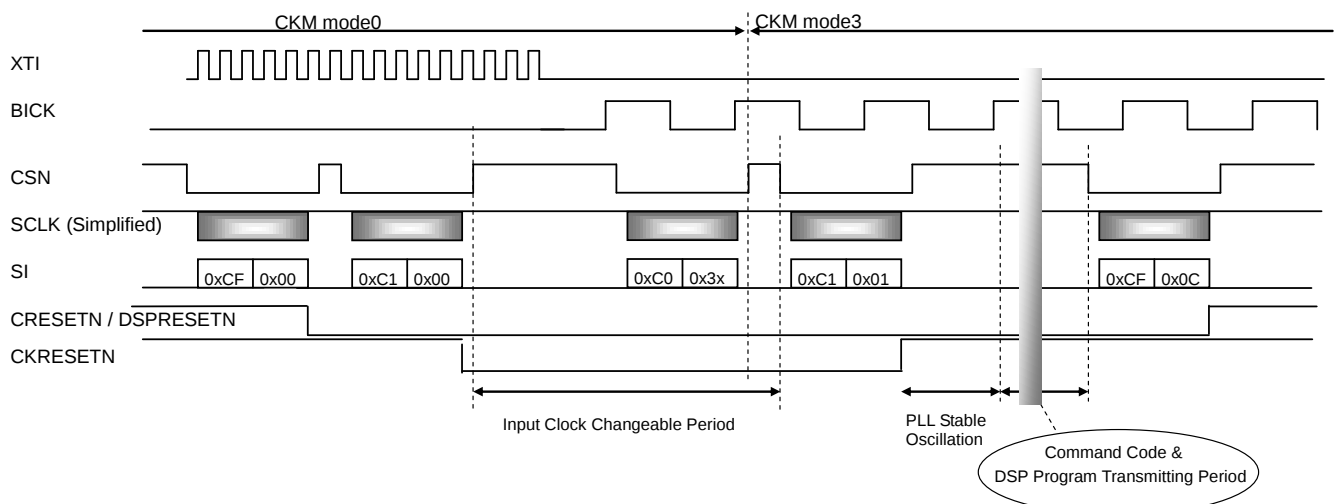
Figure 30. Clock Reset Sequence (e.g. CKM mode0 → CKM mode 3)
