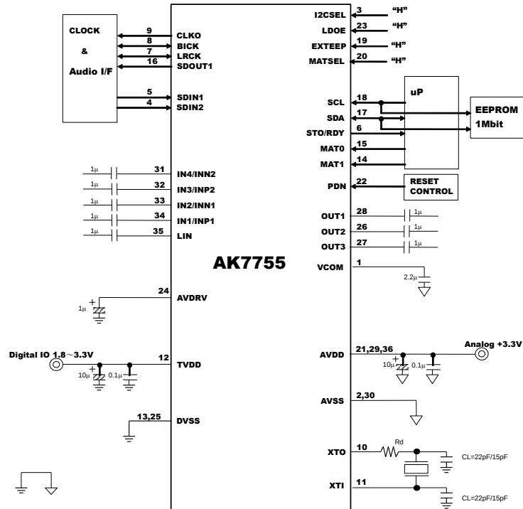
Figure 86. I 2 C Interface Connection with Internal LDO and EEPROM (Mat Select ON)
