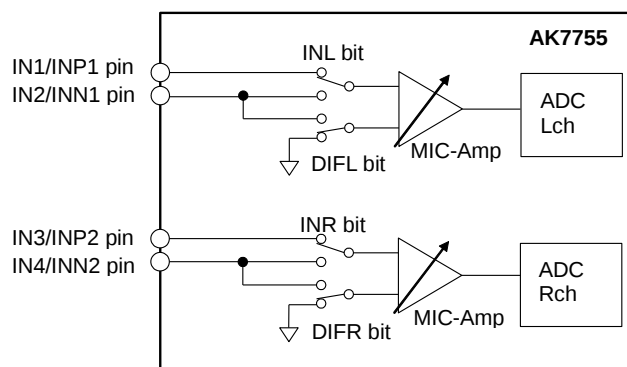
Figure 22. Analog Input Select
