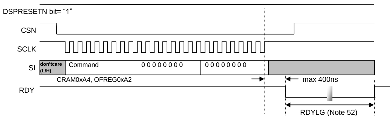
Figure 57. CRAM/OFREG Write (SPI)
