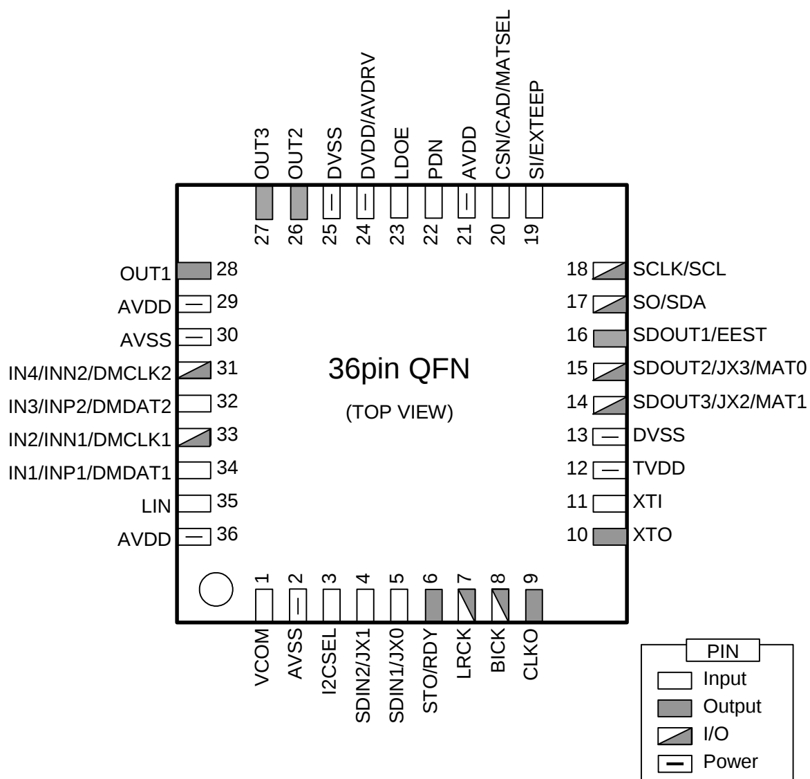
Figure 3. Pin Layout
