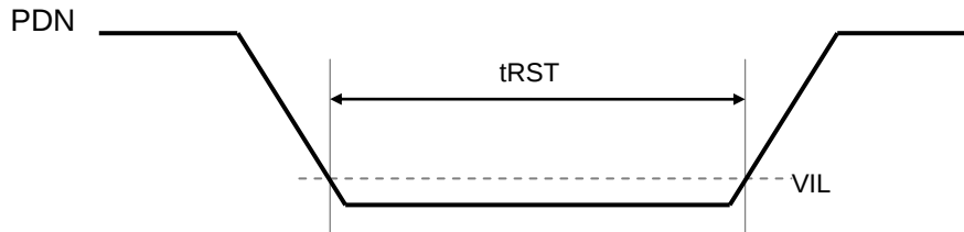
Figure 5. Reset Timing
