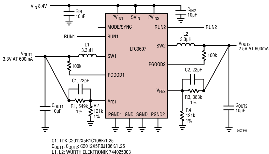
Figure 1. Design Example Circuit
