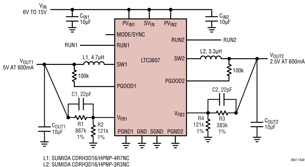
5V/2.5V 2.25MHz Buck Regulator
