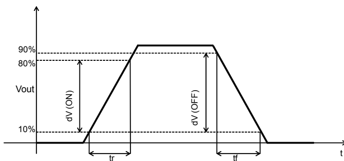
Figure 4. dV/dt
