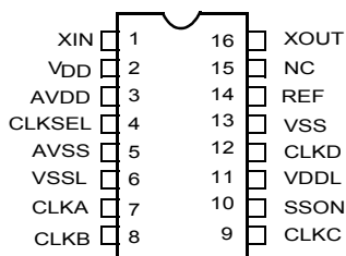
Figure 1. 16-pin TSSOP pinout
