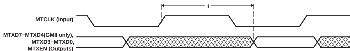
Figure 7-54. EMAC Transmit Interface Timing [MI and GMII Operation]
