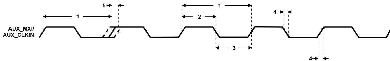
Figure 7-16. AUX_MXI/AUX_CLKIN Timing
