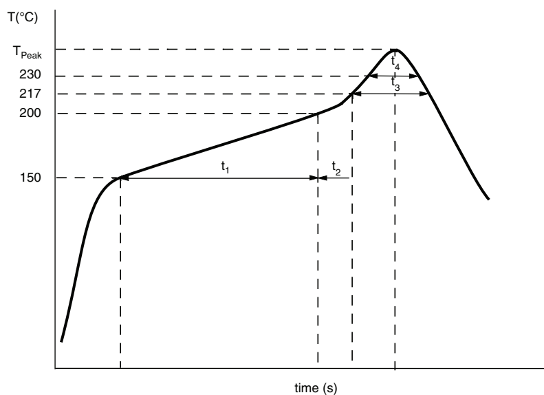
Fig.4 Maximum temperature load during reflow soldering measured on capacitors soldering pad and top of the case
