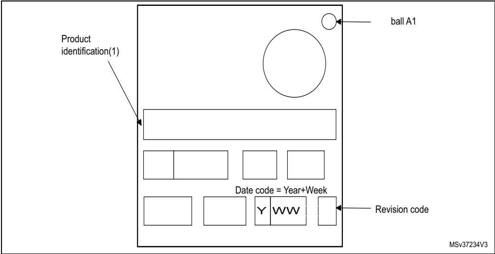
Figure 82. WLCSP143 marking example (package top view)
